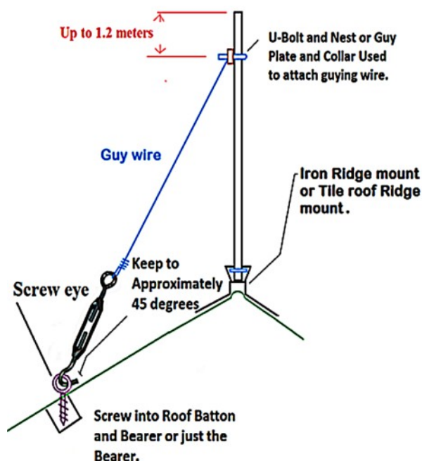
Example shown of the Screw Eye use as a Guying Wire Anchor point.
